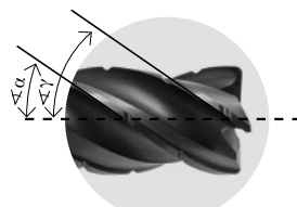
eliche differenziate different helices
