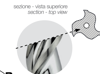
gola raggata rounded flute
