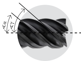
eliche differenziate different helices
